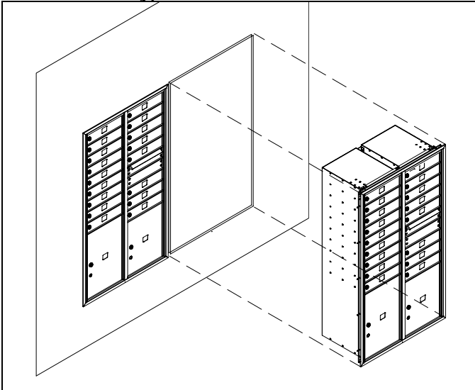
Illustration 1 - Typical Installation
