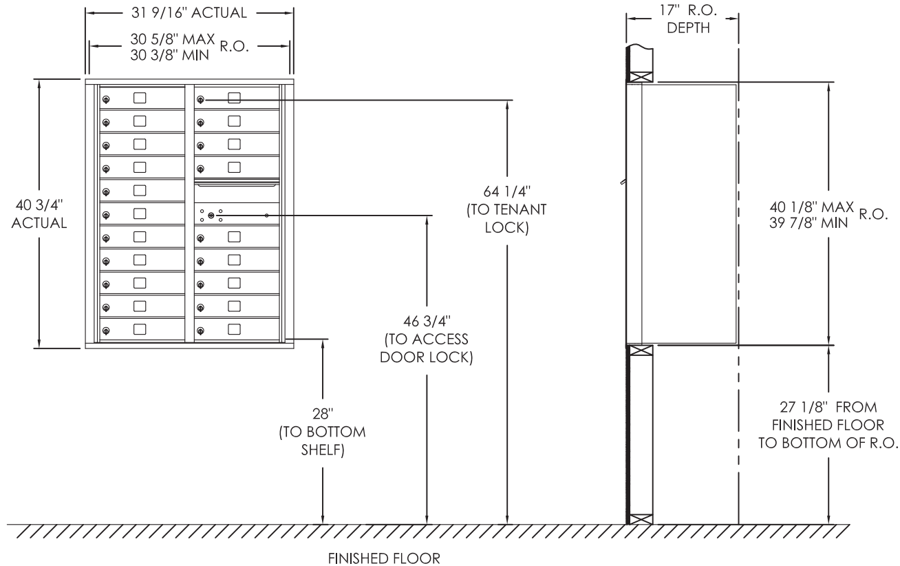
COMPARTMENT CHART
