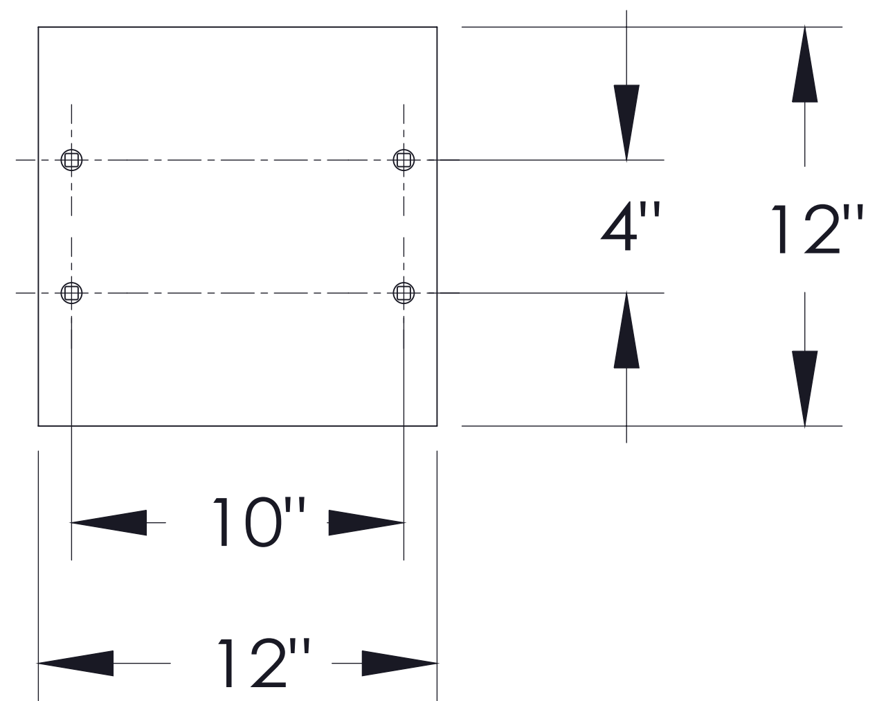
PEDESTAL BASE BOLT PATTERN
