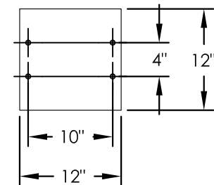
PEDESTAL BASE BOLT PATTERN
