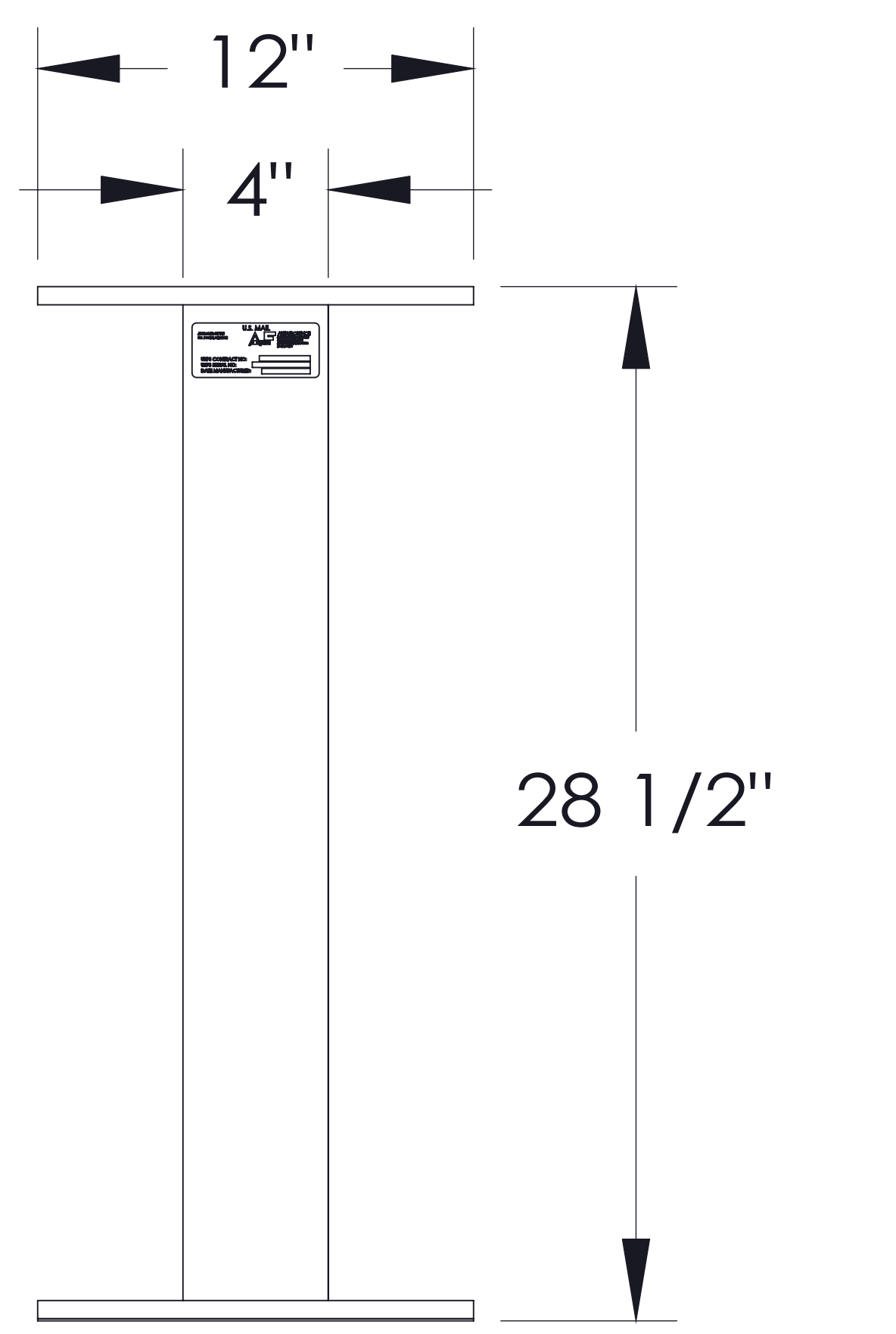
PEDESTAL
